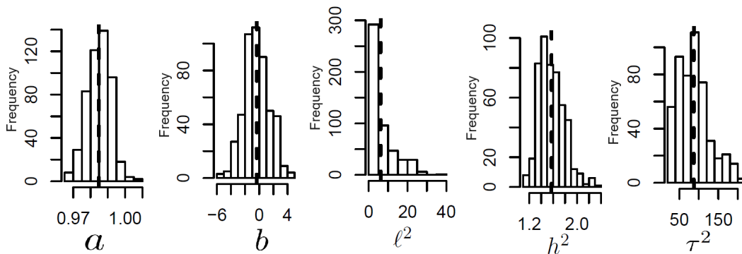
Figure 4. Summary of the posterior distribution for the stochastic volatility model via Gaussian process applied to Petrobras returns
